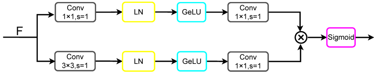
Figure 8. Improved SAM mechanism.
