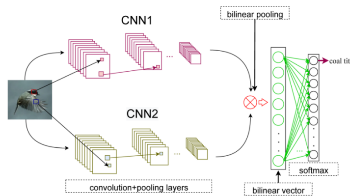
Figure 1. Structural schematic of a BCNN [19].
