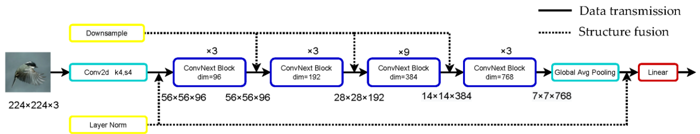
Figure 3. Network structure chart of ConvNeXt-Tiny.
