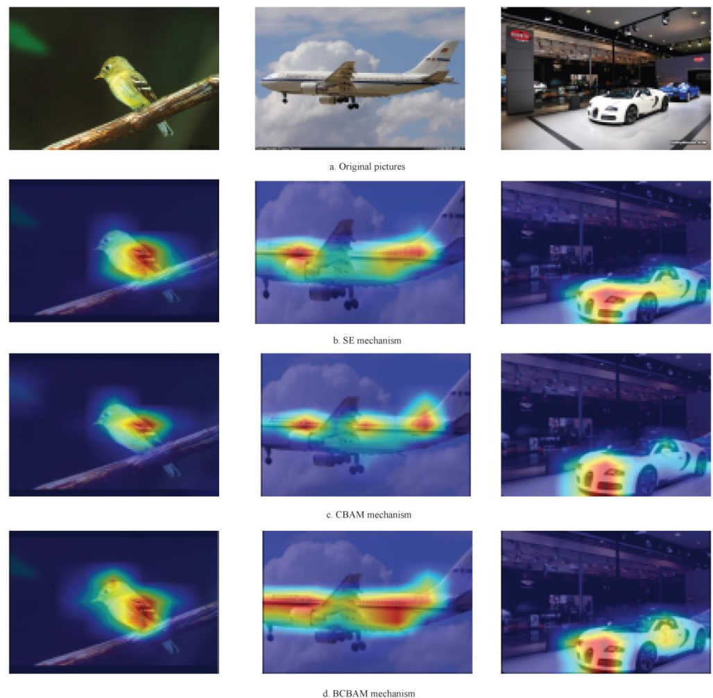
Figure 16. Thermodynamic diagrams of the three attention mechanisms.
