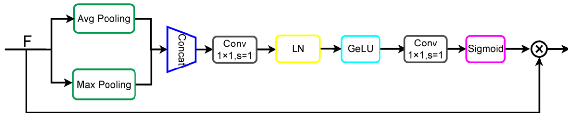
Figure 7. Improved CAM mechanism.
